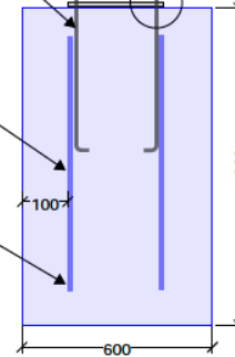
FOOTING SECTION
