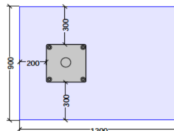
FOOTING PLAN
