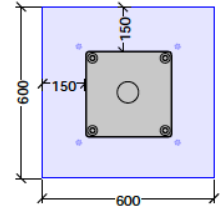
FOOTING PLAN
